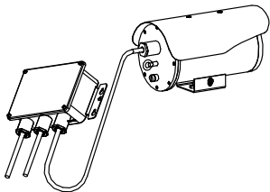
Figure 2-11 Fix the Junction Box
