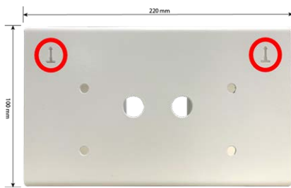
Fig. 10: Dimensions MOBOTIX c71 Corner/Pole Mount – front view
