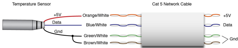
Recommended connections using Cat5 cable
